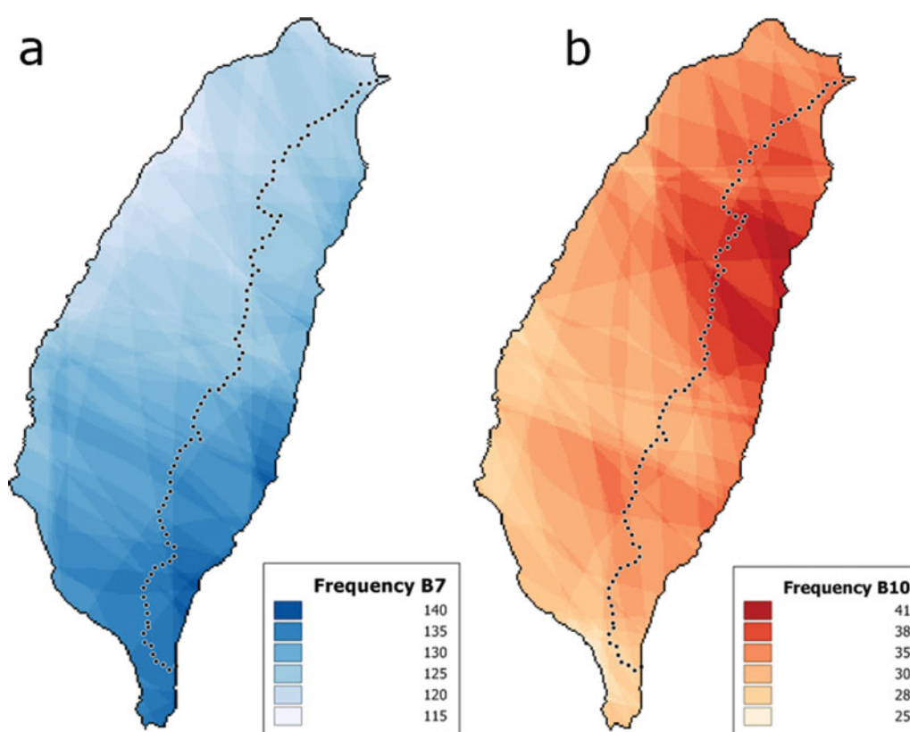
Figure 3. Typhoon frequencies in Taiwan from 1958–2006 in 1-km 2 grid cells, 167 typhoons in total (data from Taiwanese Central Weather Bureau). Tracks and eyes of typhoons were plotted as circles with radii of wind speed Beaufort scale 7 (B7) and 10 (B10) and the accumulated number of hits in each cell was calculated for both wind-speed cohorts, yielding two cyclone frequency maps (a: B7 and b: B10) as a proxy for cyclone disturbance. The dotted line on each map indicates the highest point in the central mountain range of Taiwan and only the area east of this line was analysed in this study.
